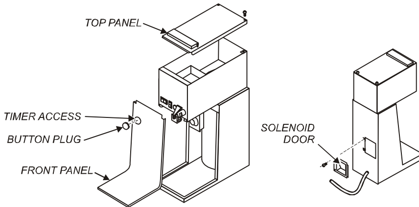
Fig. 9 Access Panels
