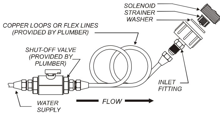
Fig. 2 Water Supply Installation - New-Style Brewers
